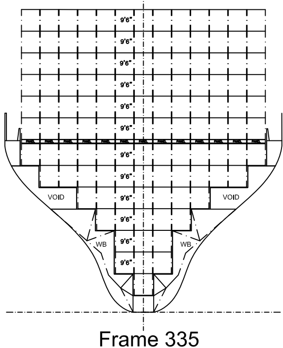
Frame 335
