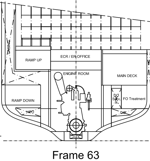
Frame 63
