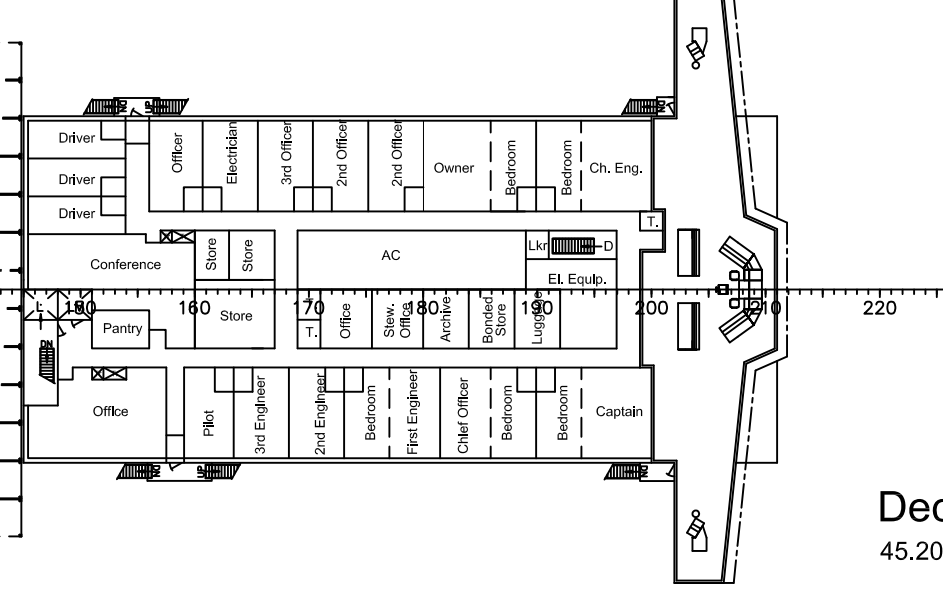
Deck 6A 37,500 m abv BL
